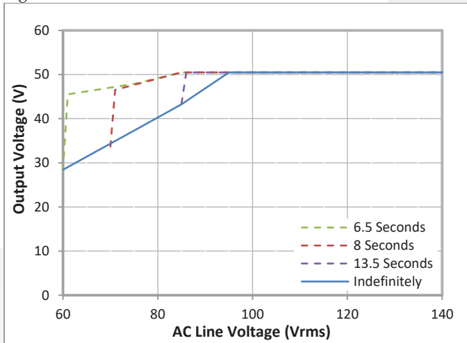
Figure 8: Full Load Output Voltage (Droop model) during Line Brownouts
