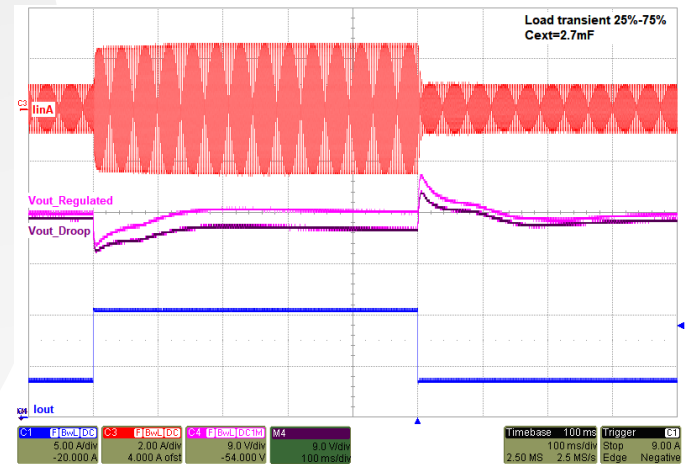
Figure 10: Responses to 25%-75%-25% Load Transient Steps: C_{ext}=2.7mF , both Regulated and Droop models.
